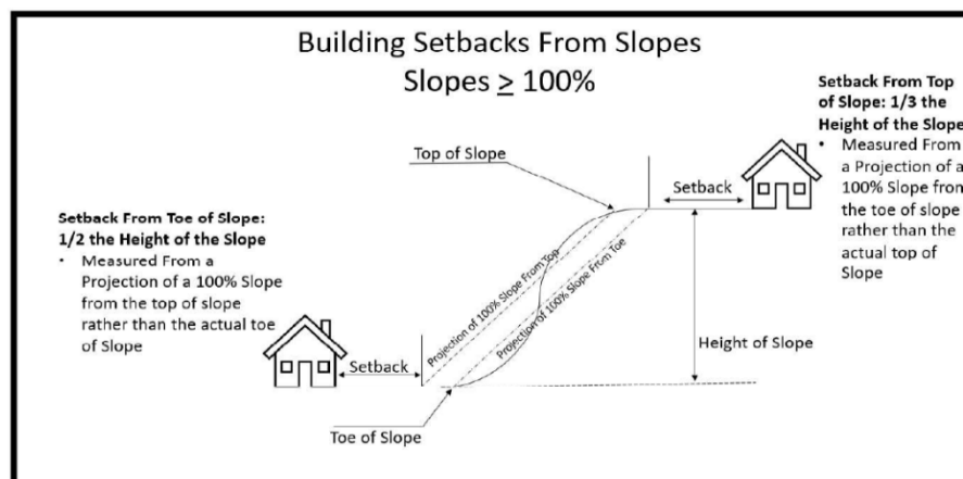
Figure 20.93.640-2: Building Setbacks From Slopes ≥ 100%
