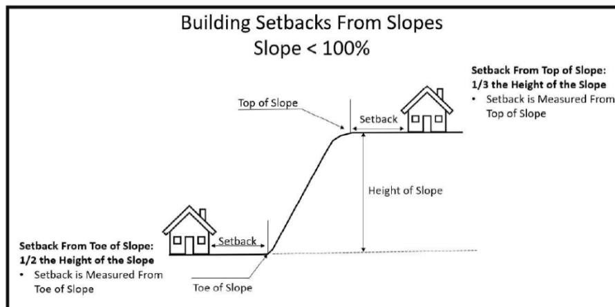
Figure 20.93.640-1: Building Setbacks From Slopes < 100%
